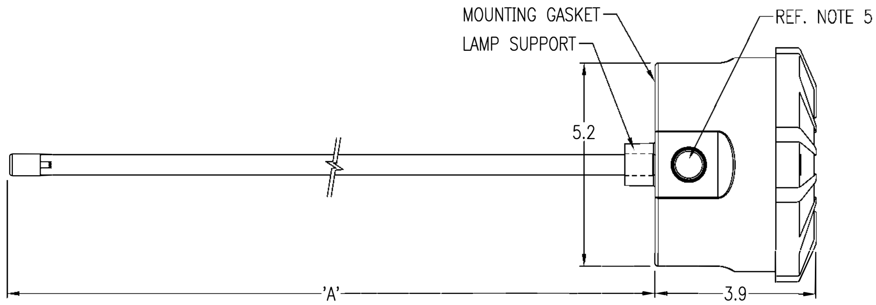
PLAN VIEW
