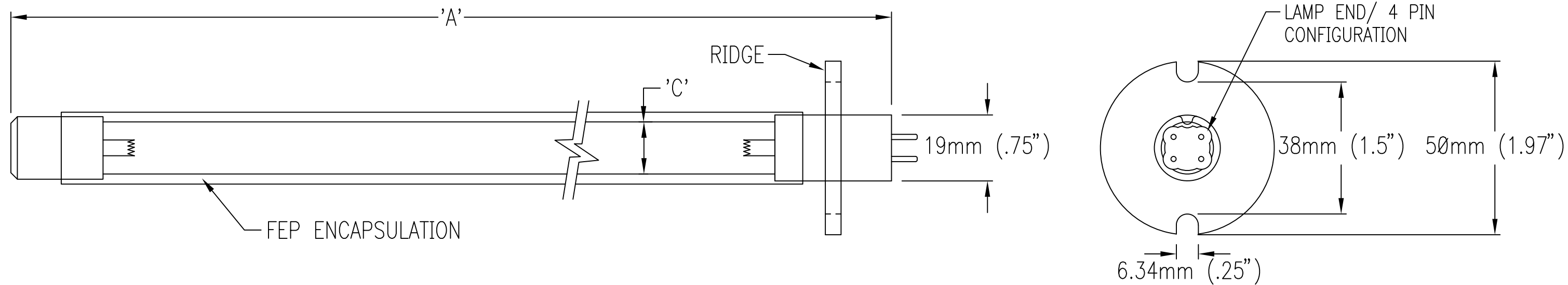
CUSTOM BASE 4 PIN SINGLE ENDED (SE) LAMPS WITH RIDGE BASE
