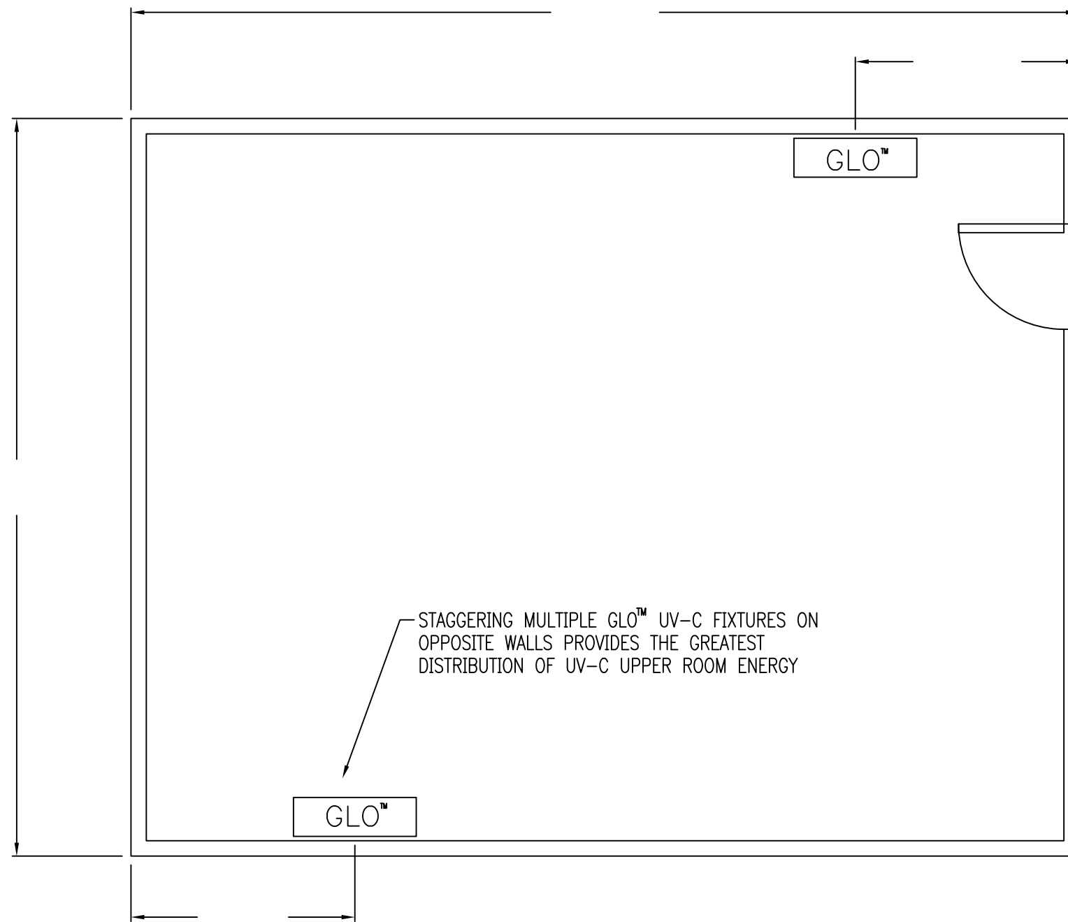
PLAN VIEW TYPICAL FIXTURE LAYOUT
