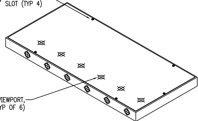
ISOMETRIC VIEW (NTS) W/ COVER INSTALLED
