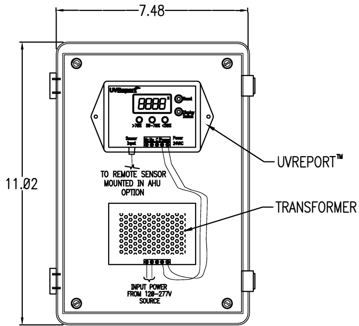
PLAN VIEW - LID REMOVED
